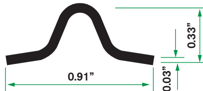
EB-CL12 dimensions
