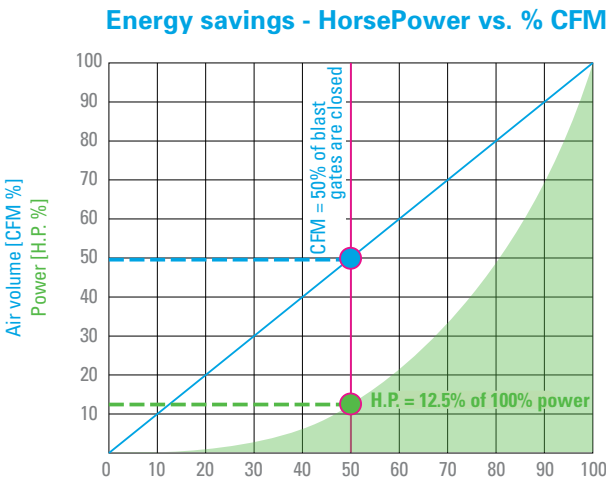
When a fan's CFM volume is reduced by 50% the kWh consumption is reduced to 12.5% of full load.
